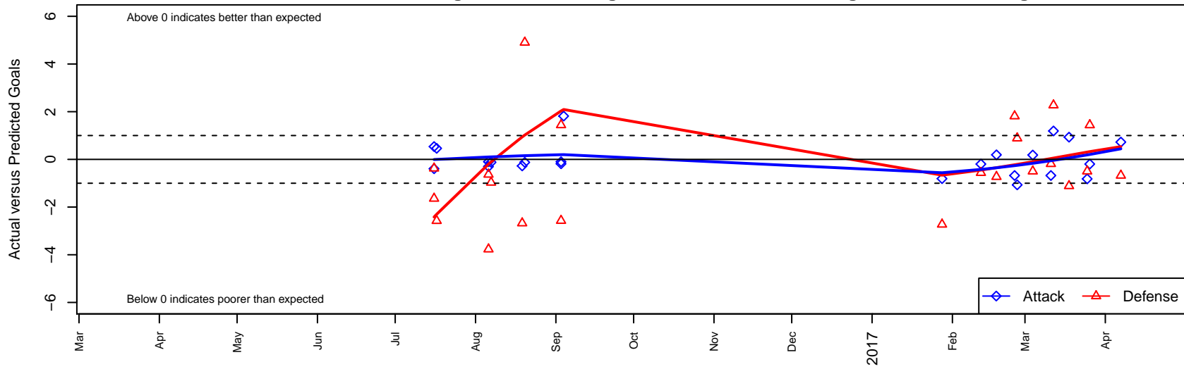
SGESC Fusion G01 Dots are actual minus expected GF (blue circles) and GA (red triangles). Blue line is smoothed change in attack strength. Red is smoothed change in defense strength.
